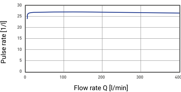
Characteristic curve
