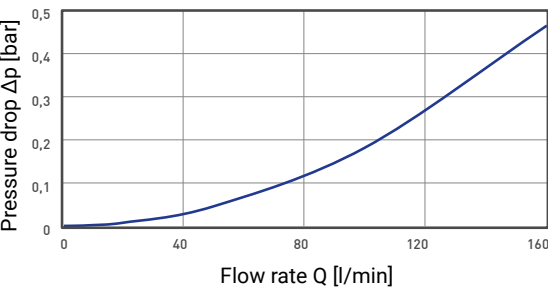
Typical pressure drop
