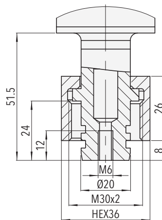
87x6.XX.2300.XX.XX.XX.XX Axial cap nut connection
