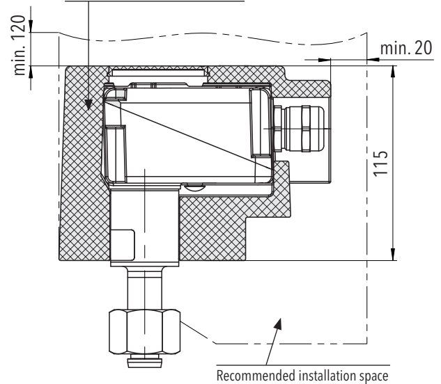
Thermal foam cover 87x6.XX.XXXX.XX.XX.XX.37
