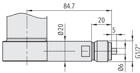
87x6.XX.1030.XX.XX.XX.XX Radial threaded connection G1/2"
