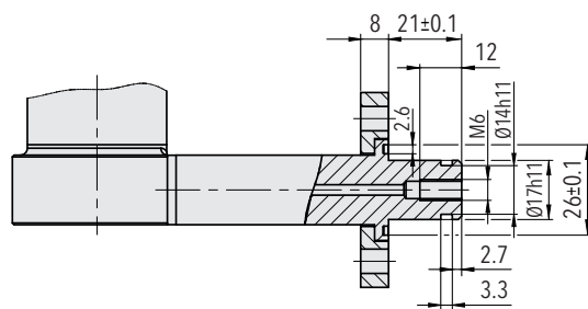
87x6.XX.2XP2.XX.XX.XX.XX Radial for two-hole flange connection
