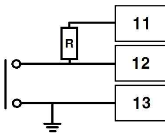
Reed Switch
