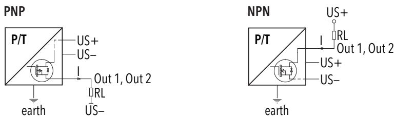
Connection of loads to switching output
